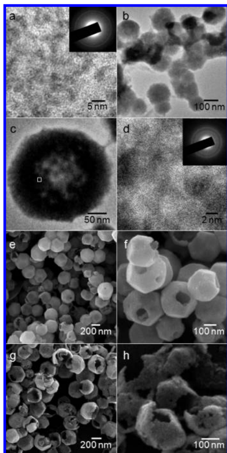
Figure 4. (a) TEM image of the small Cu 2 O nanoparticles (<5 nm) formed after aging the solution for 1 min. The inset shows the corresponding SAED pattern, which is consistent with that of cubic Cu 2 O. (b, c) Low- and high-magnification TEM images of the intermediate crystals (150–250 nm) captured after aging the solution for 10 min. (d) HRTEM image of the square region in (c), which reveals that these intermediate crystals are formed through the aggregation of many small Cu 2 O nanoparticles. The inset displays the SAED pattern of the intermediate crystal shown in (c). (e, f) Randomly etched nanocages obtained after aging the solution for 3 h without adding ethanol. (g, h) As the aging time was extended to 6 h, most of the nanocages were broken and became collapsed pieces.
